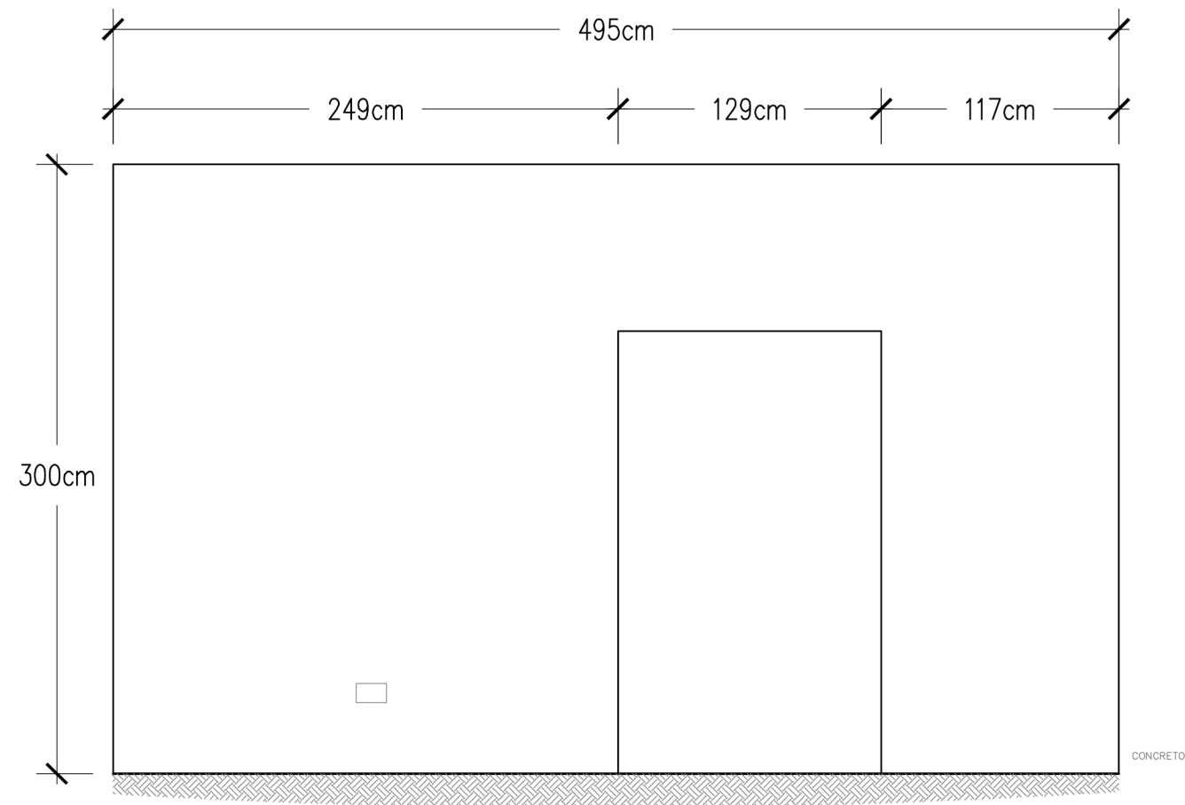
PARED 5
