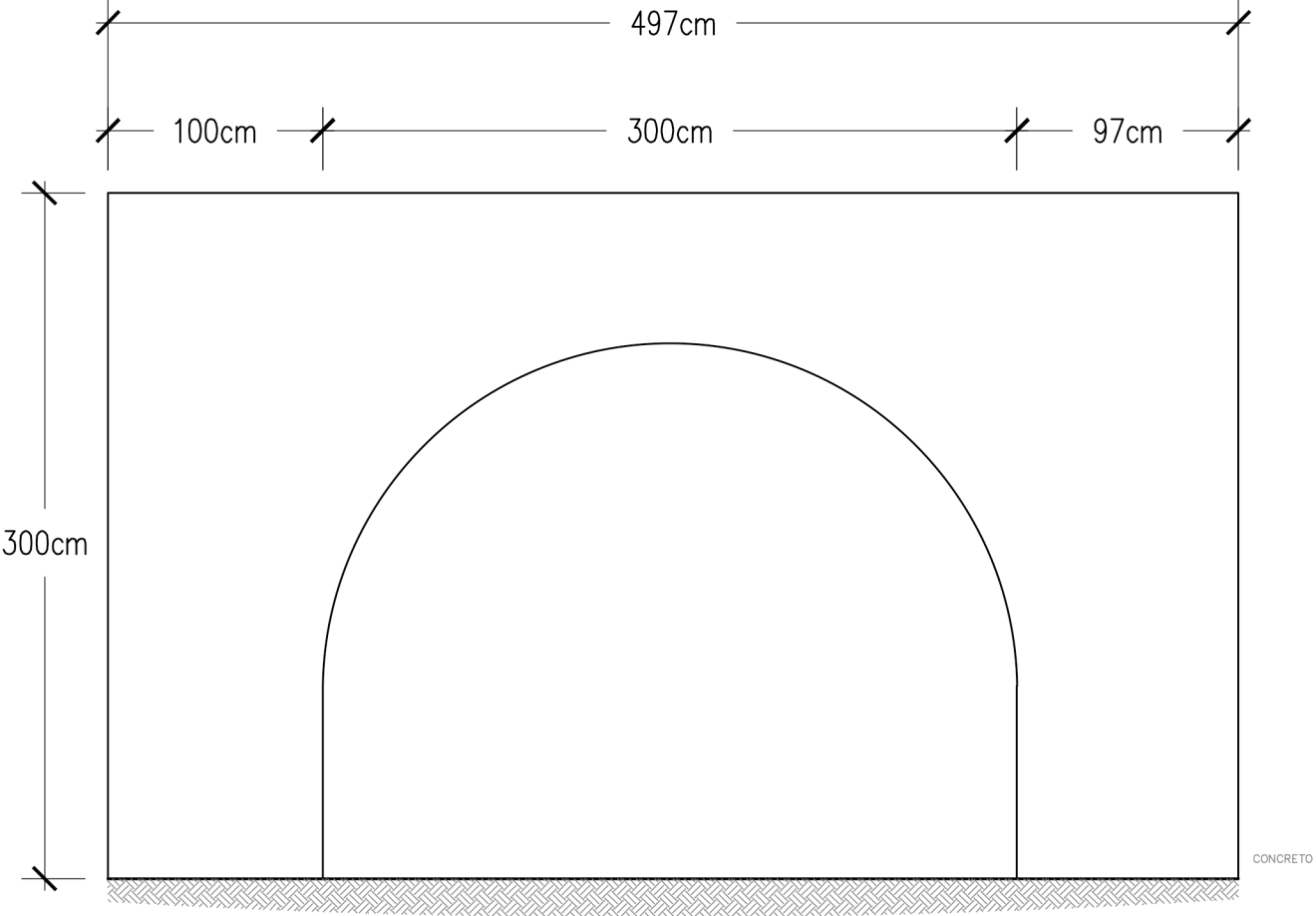
PARED 9
