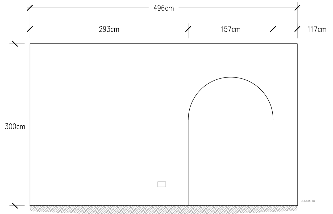
PARED 6
