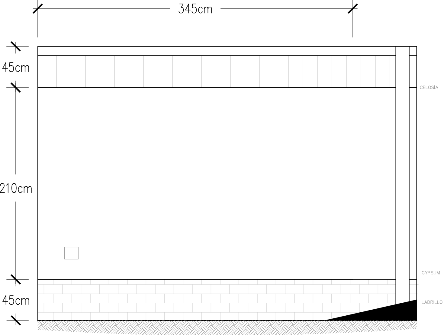
PARED 2
